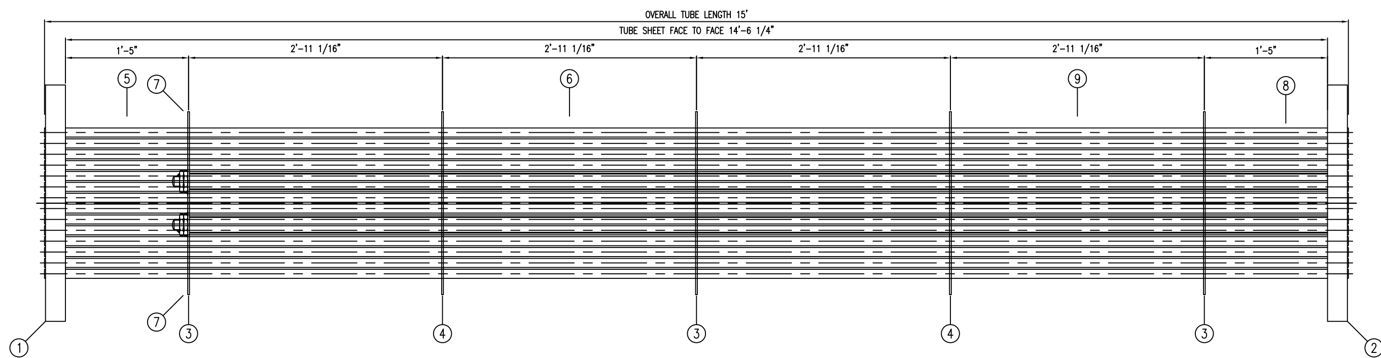
PLAN SCALE 1: 10.00 DETAILS OF TUBE BUNDLE
